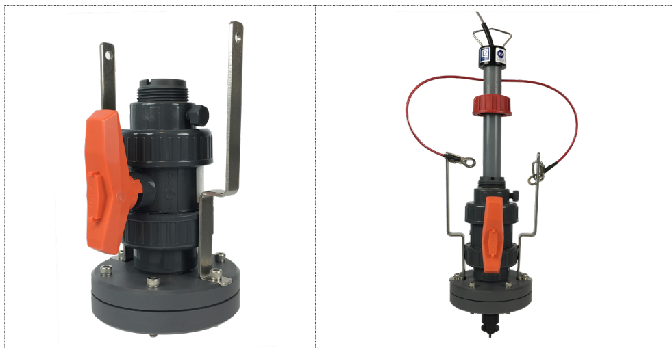
Assembly shown with extended length flow sensor installed.
