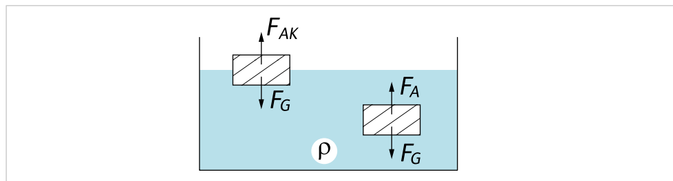
GC.28 Buoyancy
