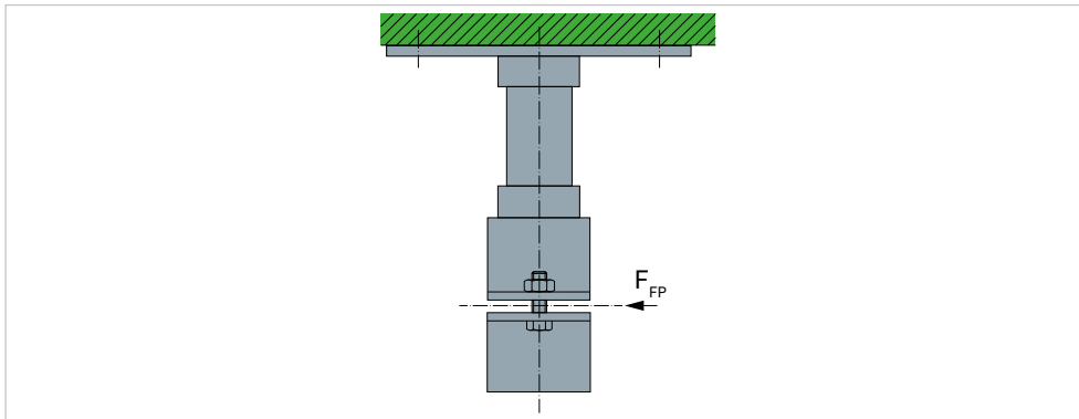
GIV.69 Determining the fixed point forces F_{FP} Fixed point force
