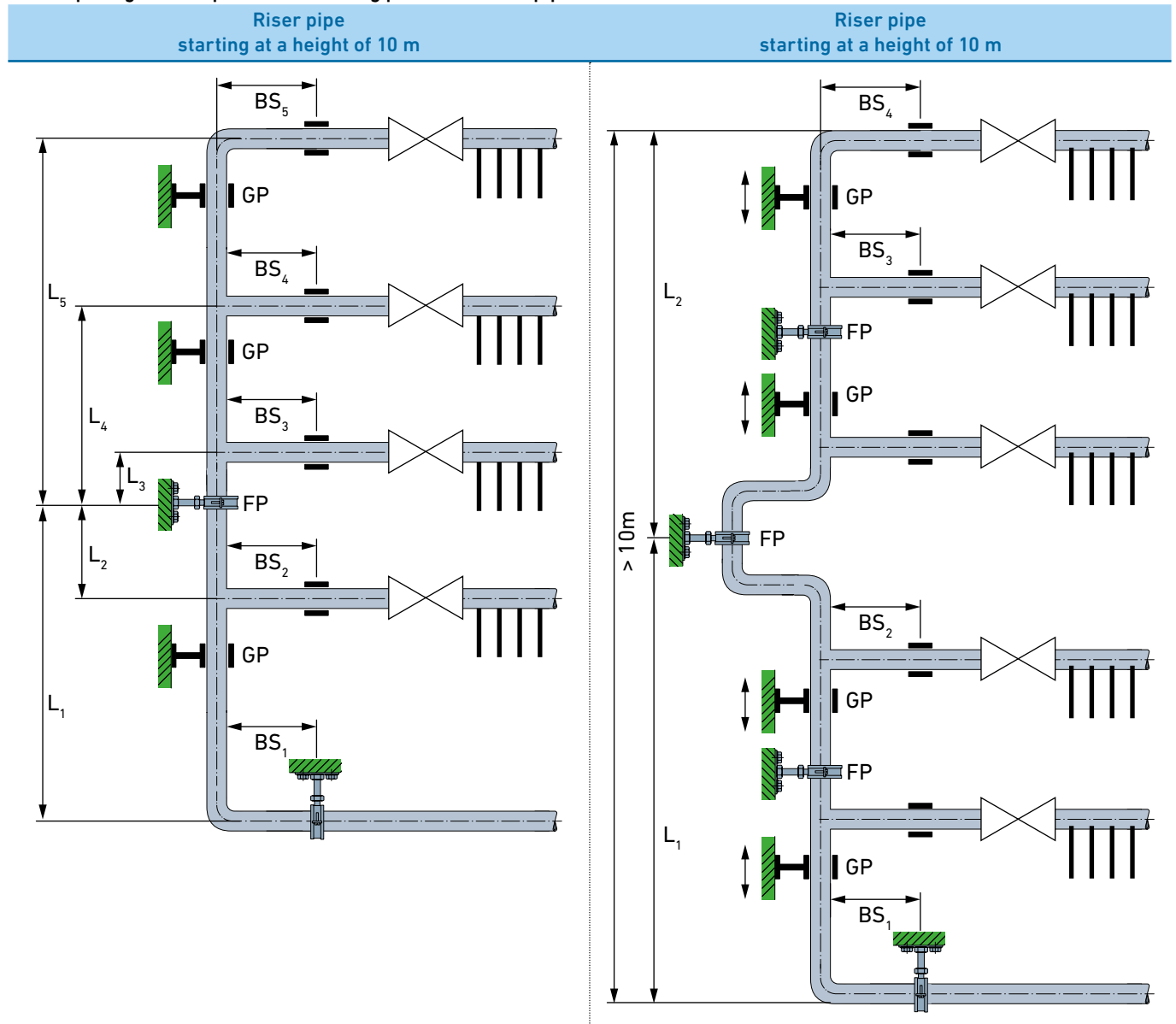
TIV.28 Spacing of fixed points and floating points in a riser pipe
