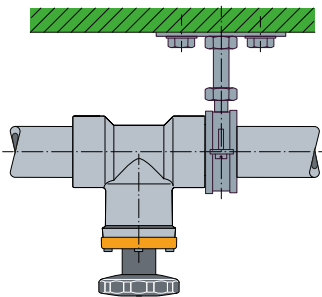
Balancing valve, horizontal installation
