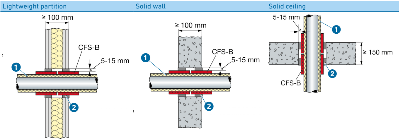
TV.48 Installation options and details
