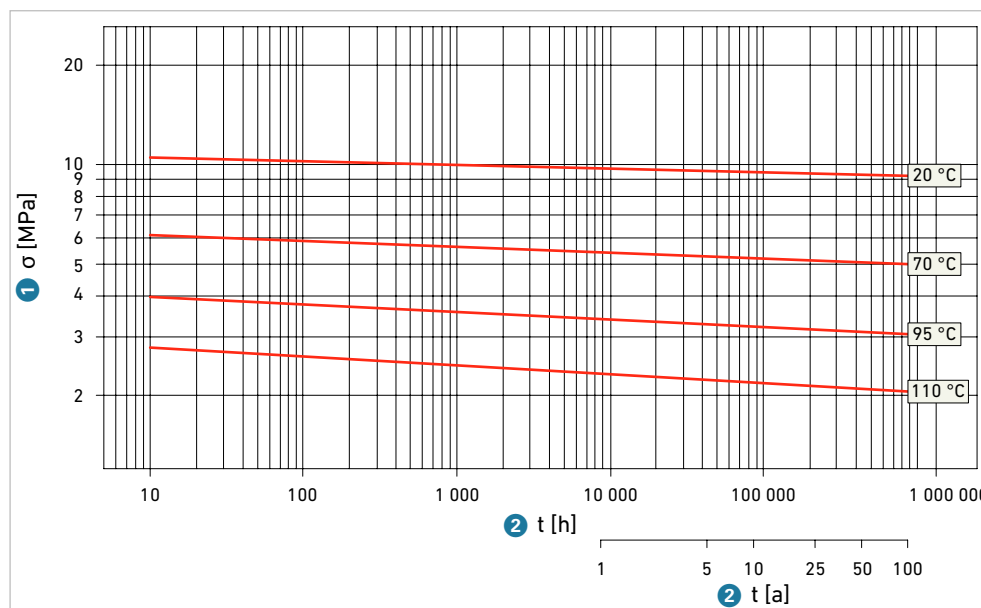
GIII.8 PE-RT, long-term creep strength
