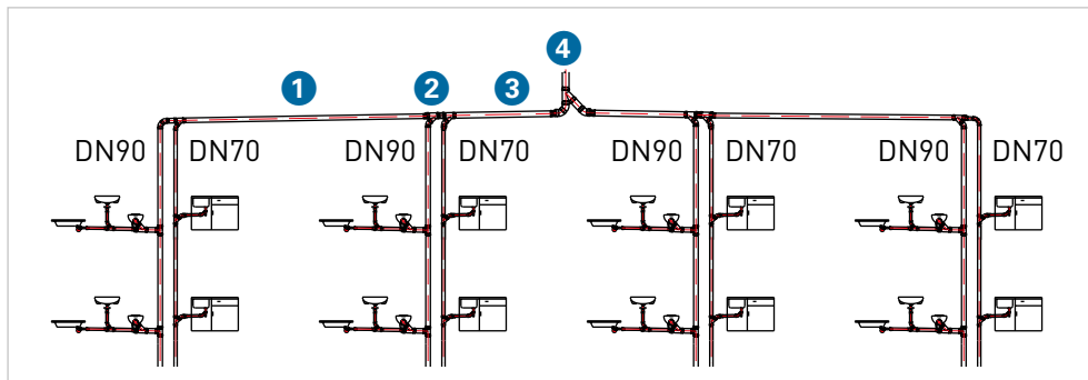
GIV.40 Dimensioning example 1 to 4: TS1 to TS4
