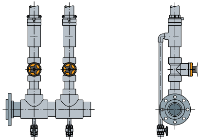
Basement distribution group without drain
