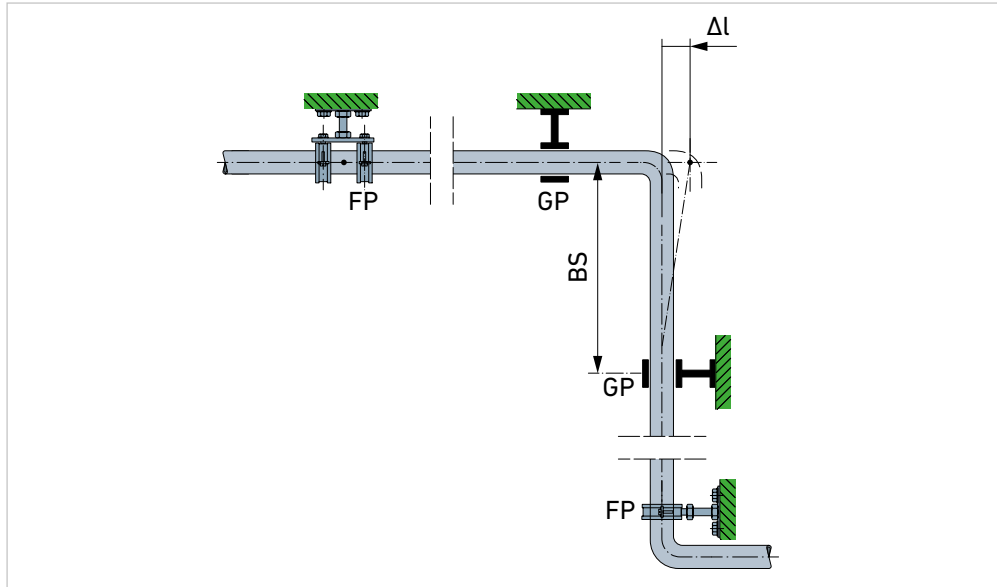
GV.25 Length of flexible pipe leg GP Floating point FP Fixed point BS Length of flexible pipe leg
