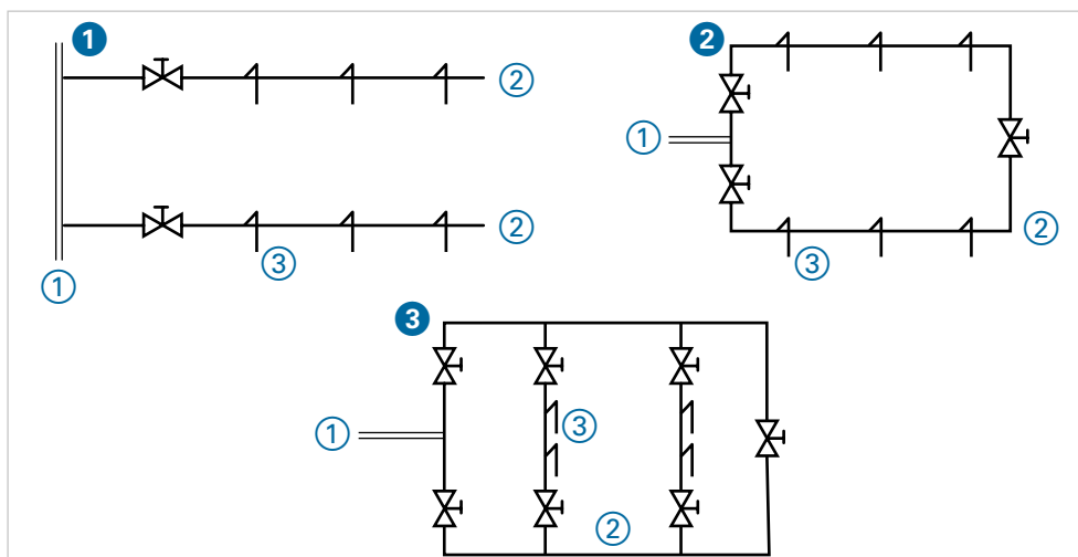
GIV.7 Types of pipelines ① Stub pipeline ② Ring pipeline ③ Ring pipeline with stub pipeline ① Main pipeline ② Distribution pipeline ③ Connecting pipeline
