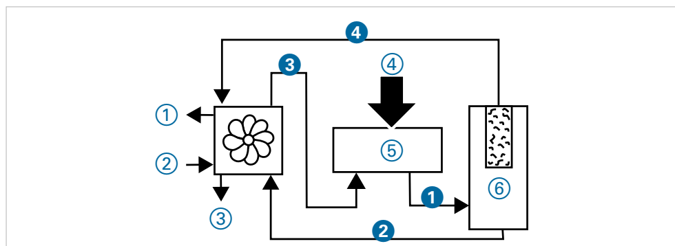
GIV.2 Compressed air production with heat recovery ① Hot water ② Cold water ③ Compressed air 5 to 10 K above ambient temperature ④ Intake air ⑤ Compressor ⑥ Oil separator ① Air/oil mixture (80/20) ② Oil with compression heat ③ cooled oil ④ Air with compression heat
