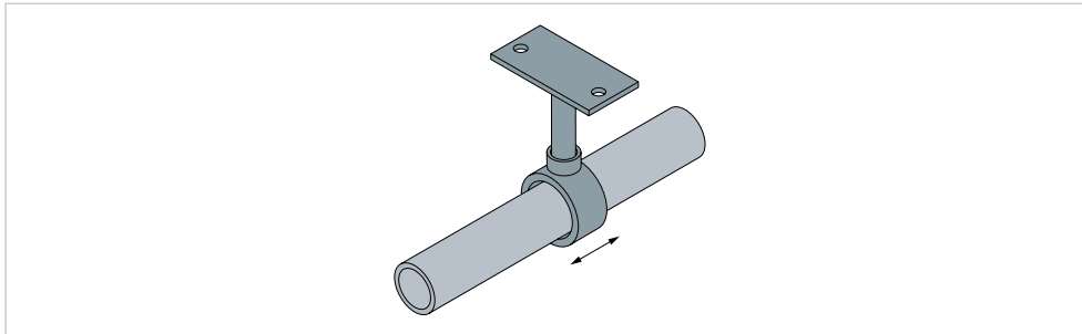
GV.37 Illustration of the pipe's mobility inside the pipe clip (floating point)
