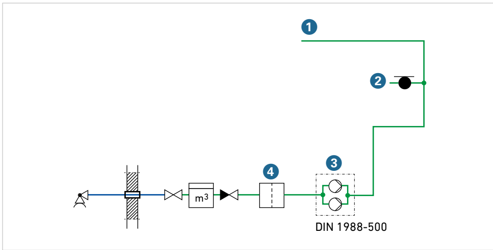
GIV.13 Drinking water installation with wall hydrant type S 1 PWC to the drinking water taps 2 Wall hydrant, type S 3 Pressure boosting system (PBS) 4 Filters
