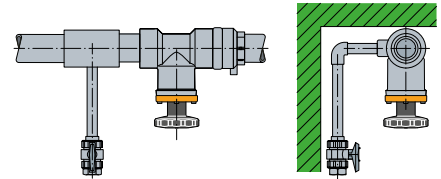
Balancing shut-off valve without drain
