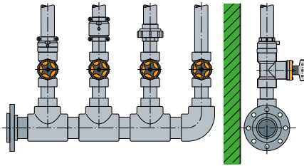
Basement distribution group up to d63
