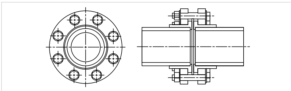
GIII.44 Alignment of the screws
