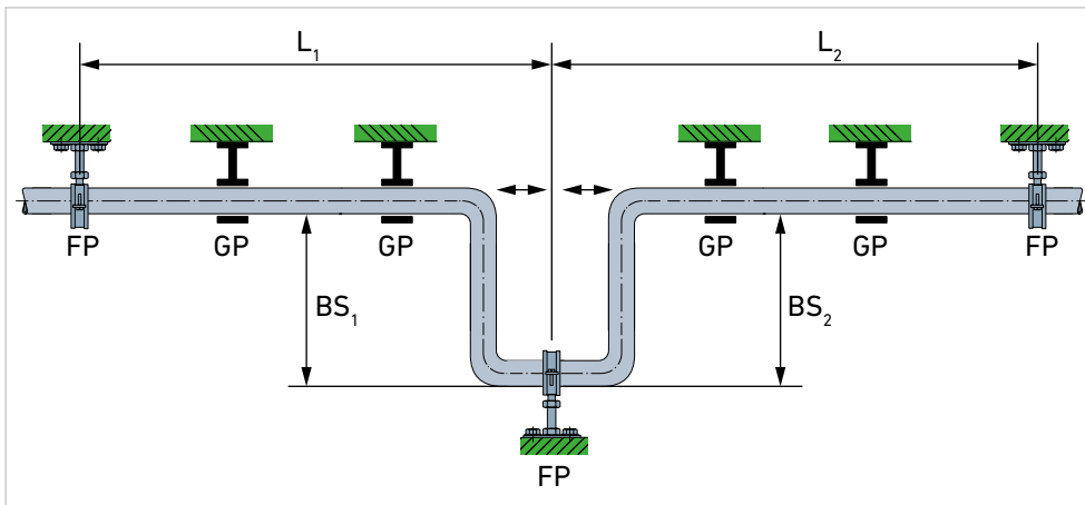
GIV.52 U-shaped expansion loop FP Fixed point GP Floating point (with sliding pipe clip) BS Flexible pipe leg l Pipe length between fixed point and deflection
