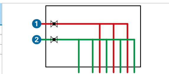
TV.3 Distributor with DHW heater water meter and shut-off valves 1 Hot water 2 Cold water
