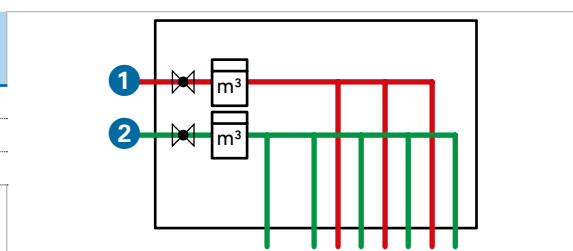
TV.5 Distributor with hot and cold water meter and shut-off valves 1 Hot water 2 Cold water
