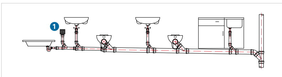
GIV.28 Ventilation valve for longer single or multiple collecting pipes 1 Ventilation valve
