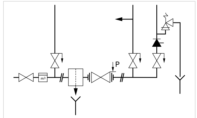
GV.17 Installation diagram
