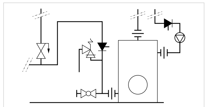
GV.35 Installation diagram
