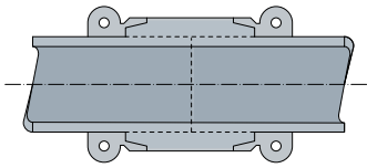
Electrofusion joint (HWS) for PB and PE
