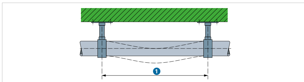
GIV.75 Pipe span and buckling length
