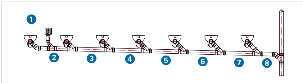
GIV.27 Ventilation valve as a replacement for an indirect secondary line or ventilation line ... in a heavily loaded collecting pipe (in-line toilet system)
