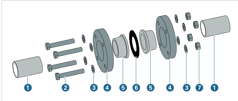
GIII.42 Flange connection
