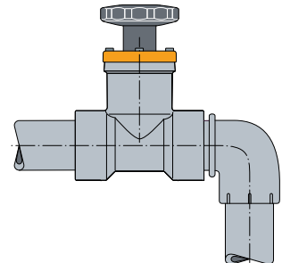
Balancing valve with welded in fitting
