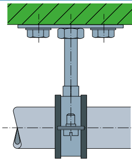
Fixed point attachment d63
