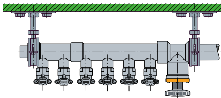
PB valve with multiple distributors
