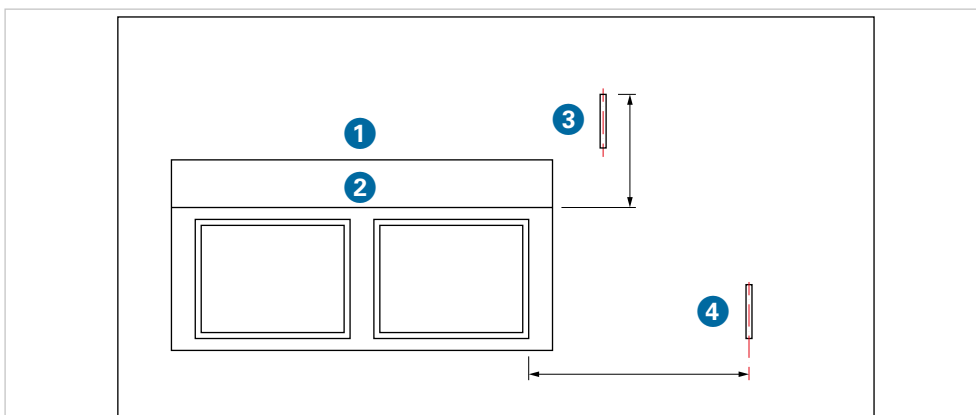
GIV.30 Minimum clearances of the endpipes from ventilation pipes to windows of common rooms
