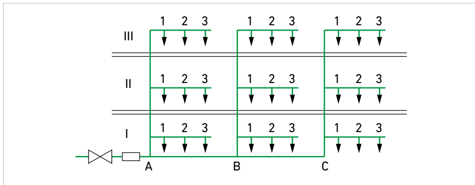
GV.3 Flushing sequence A ... C Riser pipe I ... III Floor level 1 ... 3 Tap
