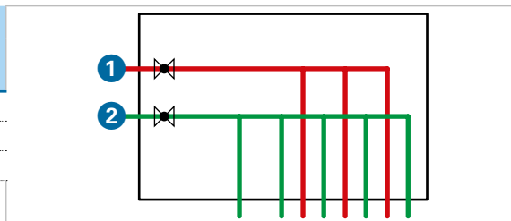
TV.8 Distributor with DHW heater water meter and shut-off valves 1 Hot water 2 Cold water
