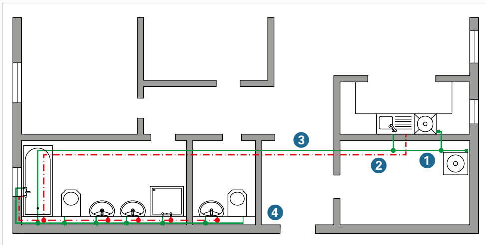
GIV.37 Floor plan of a flat with cold water pipe in the floor structure and underfloor heating
