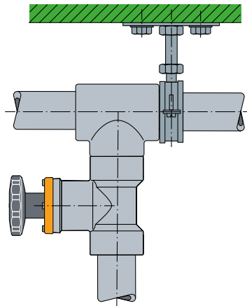
Balancing valve with HWS transition (e.g. when using riser pipes)
