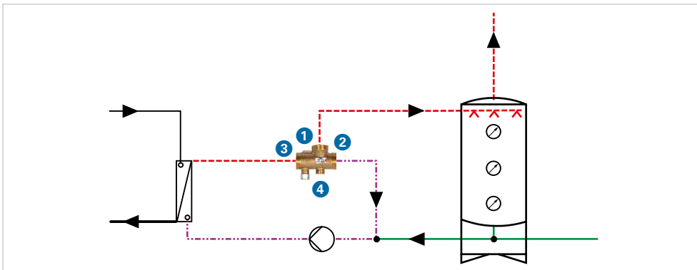
GV.32 Mixed water installation 1 Cold water inlet 2 Hot water inlet 3 Mixed water outlet 4 Circulation inlet with end cap 8325
