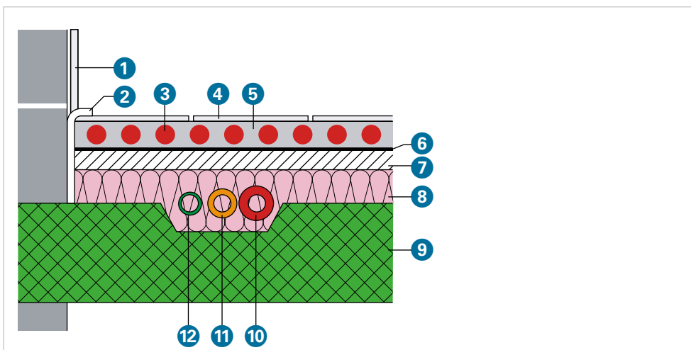
GIV.38 Floor structure
