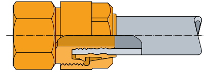
Clamp connection for PB
