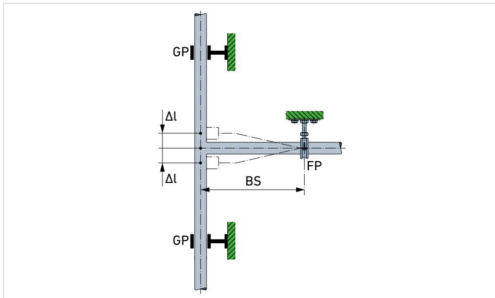
GV.26 Length of flexible pipe leg GP Floating point FP Fixed point BS Length of flexible pipe leg
