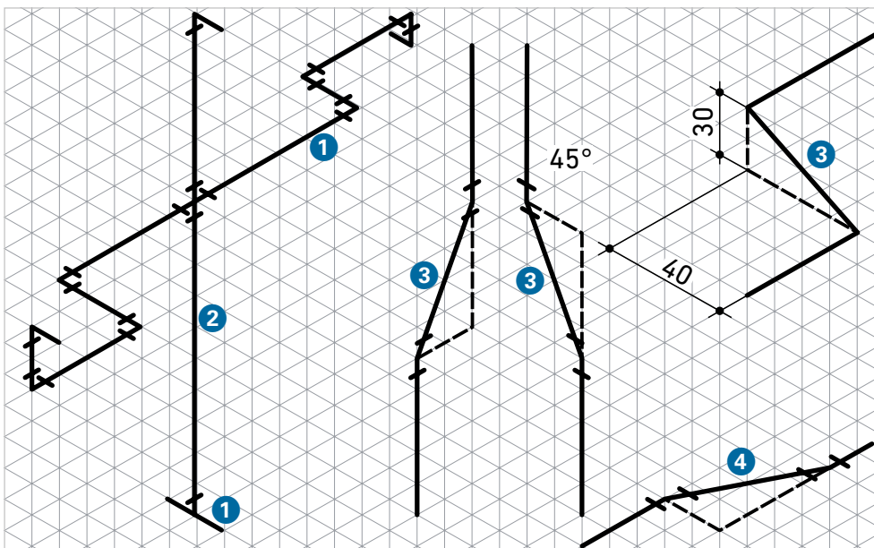
GIV.89 Sketching directional changes
