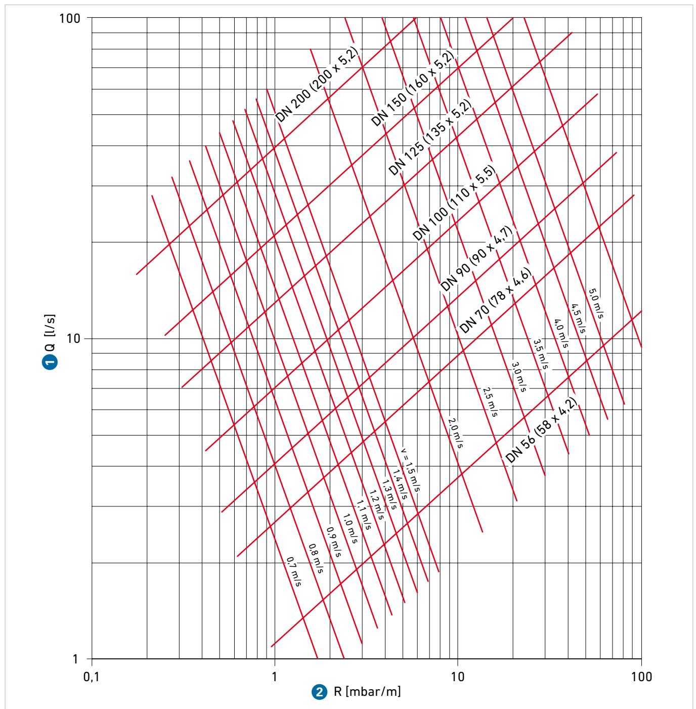
GIV.38 Pressure loss diagram for Silenta Premium pipelines
