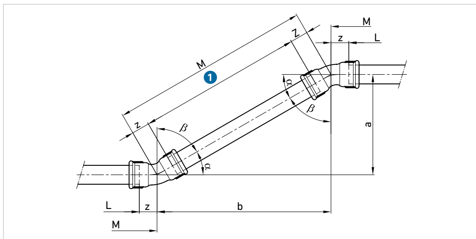
GIV.87 Dimensions M and L if using oblique pipelines
