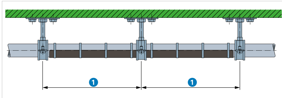
GV.24 Mounting distances ( BA ) 1 Mounting distance
