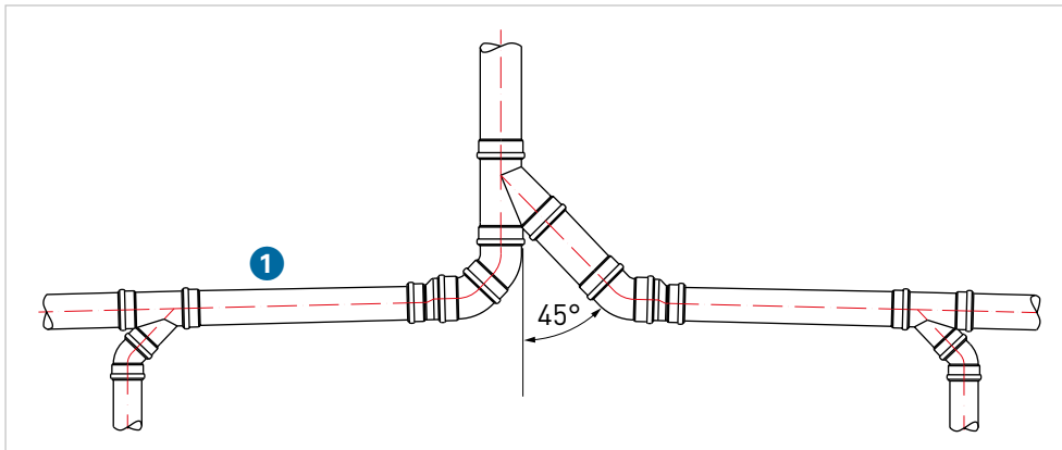
GIV.26 Merging main ventilation pipes into collecting ventilation pipes 1 Slope J > 2 \text{ cm/m}
