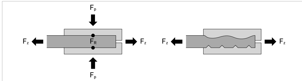
GIII.34 Effect of forces in a clamp connection
