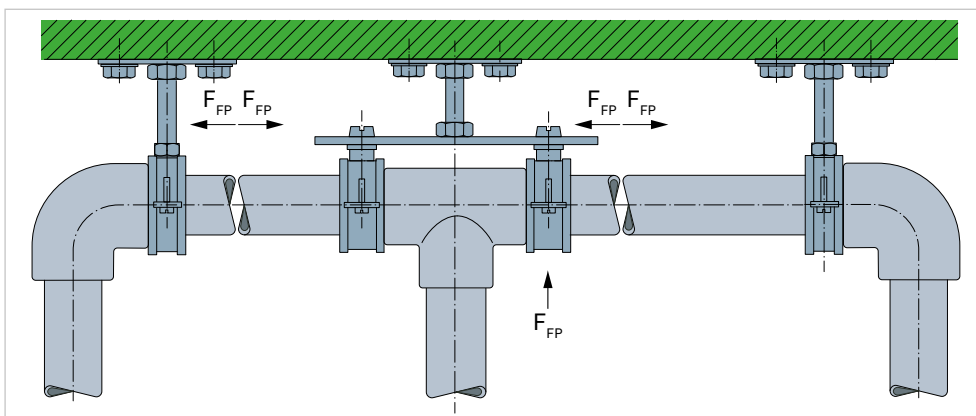
GIV.71 Variant F_{FP} Fixed point force
