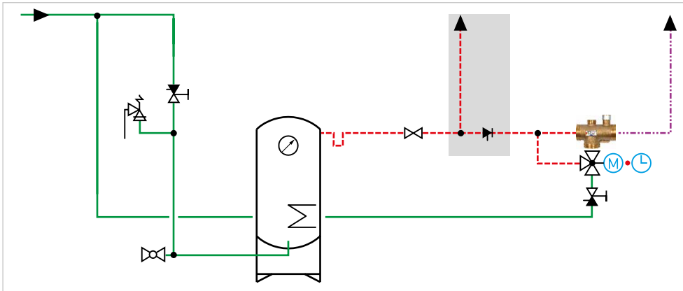
GV.30 Mixed water installation, option: Hot water outlet
