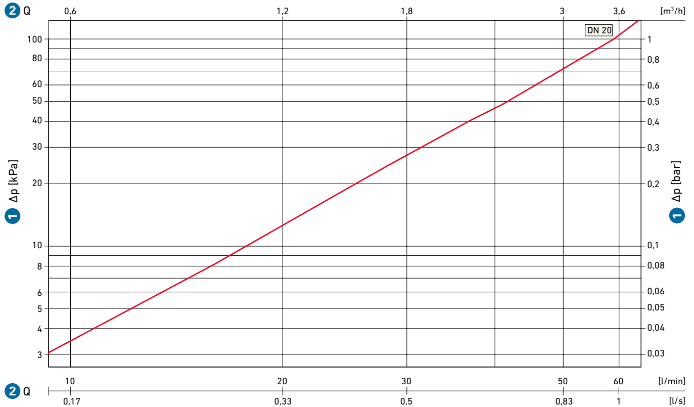
JRG LegioStop Concealed shut-off fitting 5916, without KOAX counter connection
