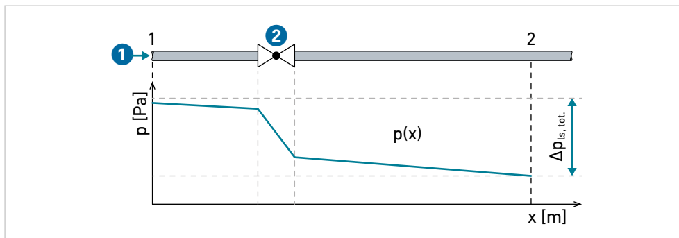
GC.32 Pressure loss 1 Flow direction of the fluid, e.g. water 2 Built-in fixtures: e.g. valve, fitting, instrument 1 Condition at the start 2 Condition at x p Pressure p(x) Pressure loss along distance x x Pipe section (pipe length [m])
