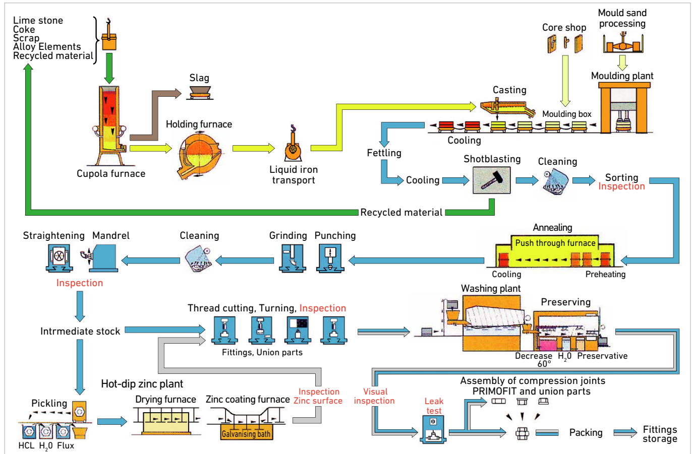
GIII.16 Production of malleable iron
