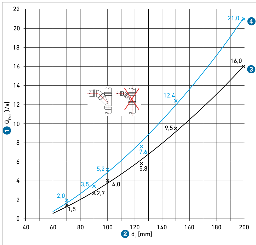
GIV.33 Drainage capacity of downpipes ...depending on the diameter and the inlet geometry of the branch 1 Drainage capacity of a downpipe 2 Internal diameter of the downpipe 3 Branches without inner radius 4 Branches with inner radius
