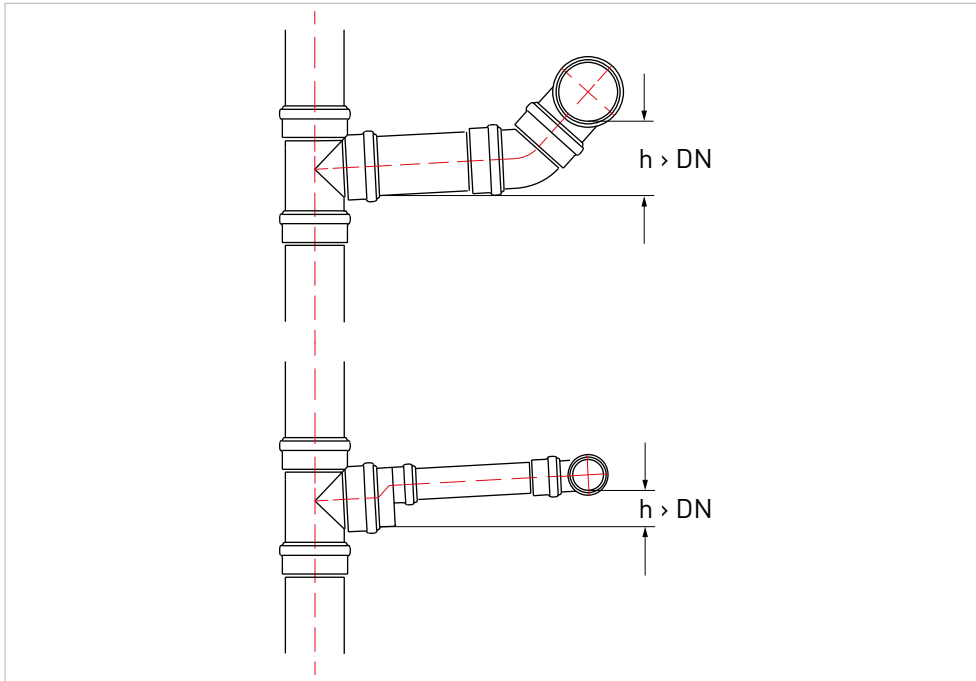
GIV.13 Minimum height difference "h" required ...between the water level in the odour trap and the invert of the connection line at the downpipe branch
