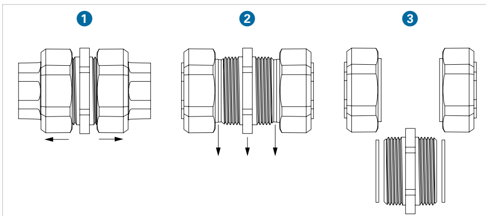
GV.9 Loosening a flat sealing service fitting Fig. 350
