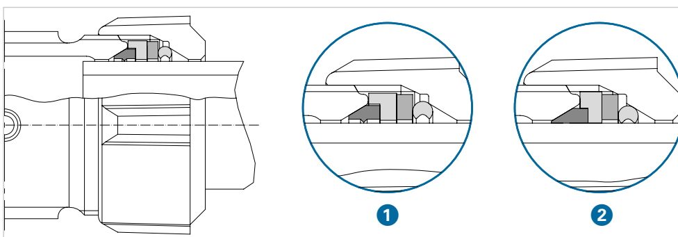
GV.3 Connection for steel pipe (HTL version) 1 Loose connection 2 Tightened connection
