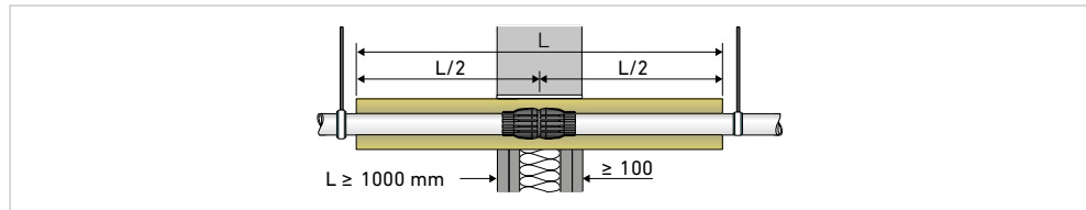
GV.18 Assembly of the JRG pipe connector
