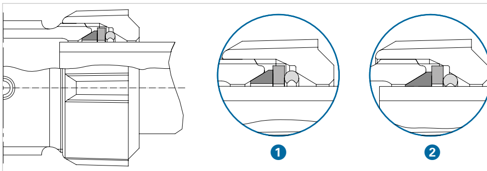
GV.2 Connection for steel pipe 1 Loose connection 2 Tightened connection
