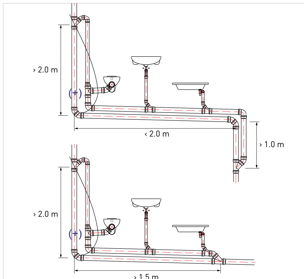
GIV.22 Connections in an area subject to critical excessive pressure or off-sets with bypass lines
