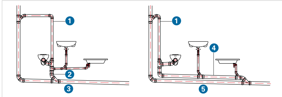
GIV.41 Dimensioning bypass and ventilation pipes 1 Ventilation pipe ≥DN70 2 Collecting pipe 3 Downpipe off-set 4 Bypass ≤DN100 5 Header
