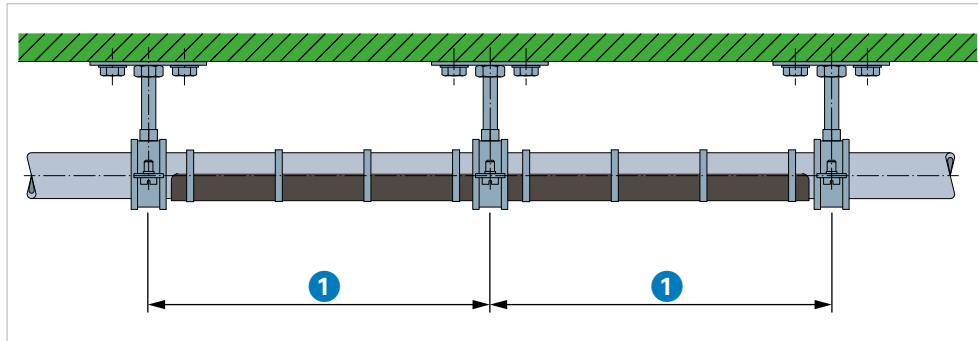
TV.47 Mounting distances (BA) 1 Mounting distance
