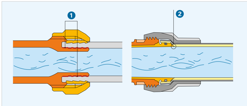
GII.17 Pipe connections without dead space 1 Dead space 2 Sealing edge, no dead space (this example shows a clamping connection with JRG Sanipex MT)
