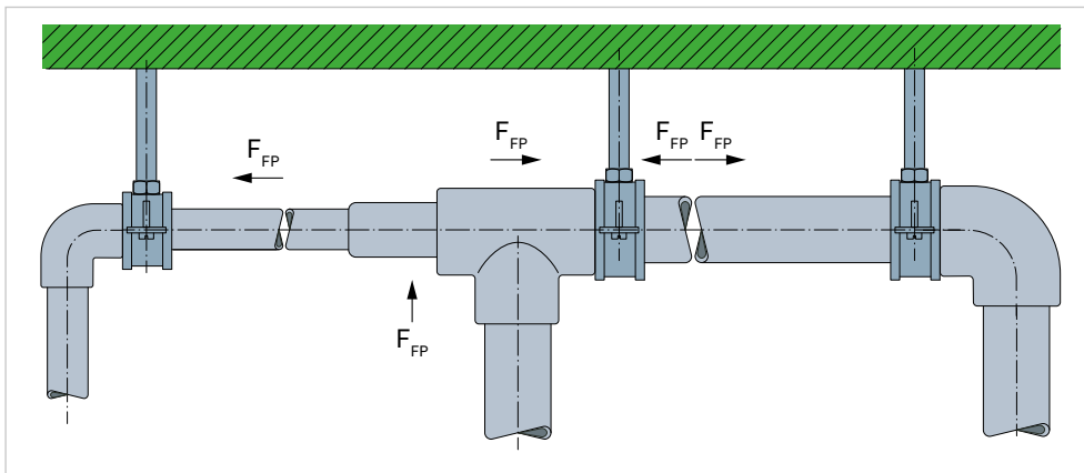
GIV.70 Fixed point if the pipeline's diameter is reduced F_{FP} Fixed point force
