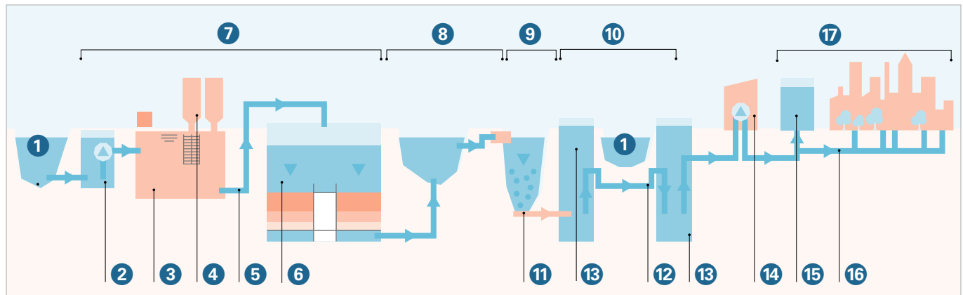
GIII.6 Drinking water production from rivers (as an example)
