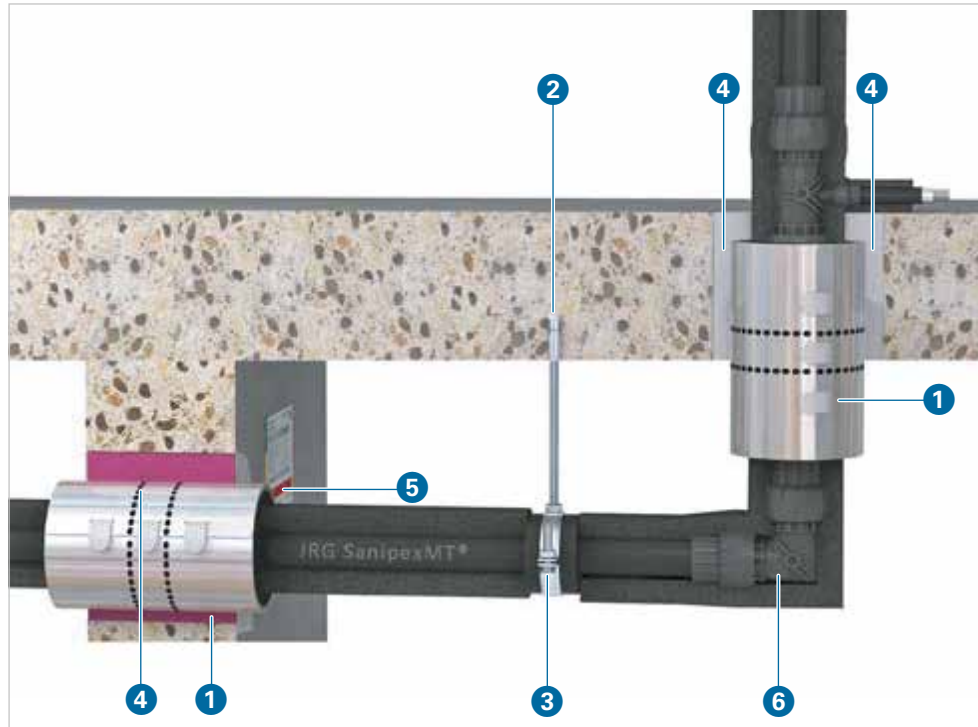
GV.20 Product overview
