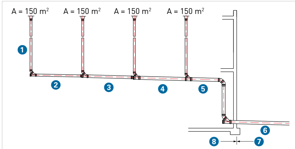
TIV.25 Design of the rainwater header in a block of flats and a commercial building
