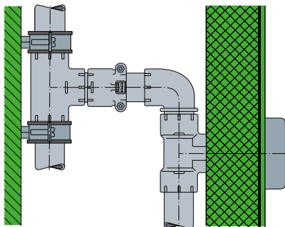
Balancing valve installed in riser pipe discharge (UP assembly incl. attachment)
