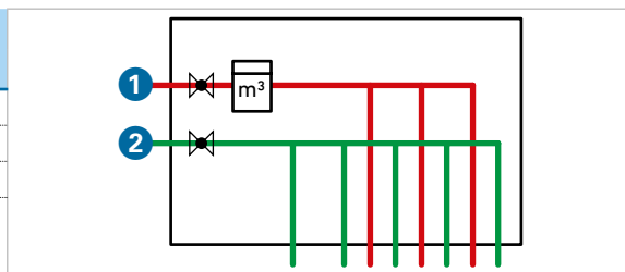
TV.4 Distributor with DHW heater water meter and shut-off valves for hot and cold water 1 Hot water 2 Cold water
