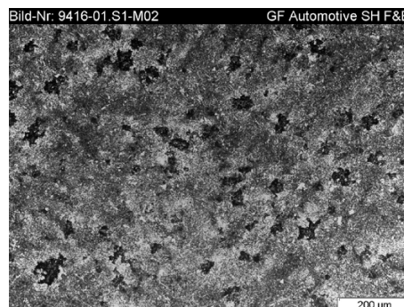
GIII.18 Black malleable iron, micrograph (etched)
