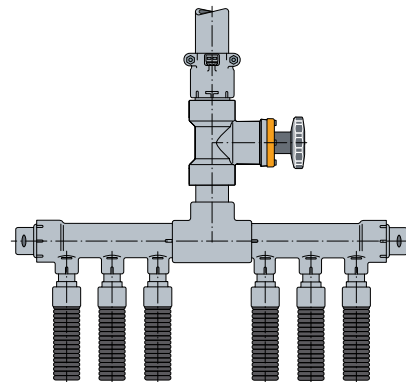
PB valve with handwheel HWS transition, double distributor
