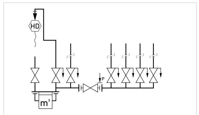
GV.36 Installation diagram
