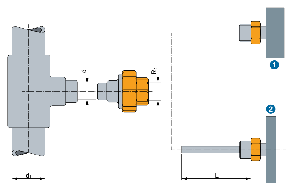
GV.6 Adaptor union 1 Pressure gauge 2 Thermometer
