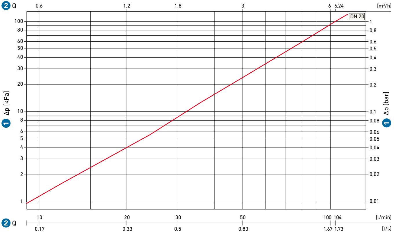
JRG LegioStop Concealed shut-off fitting 5910, without KOAX counter connection
