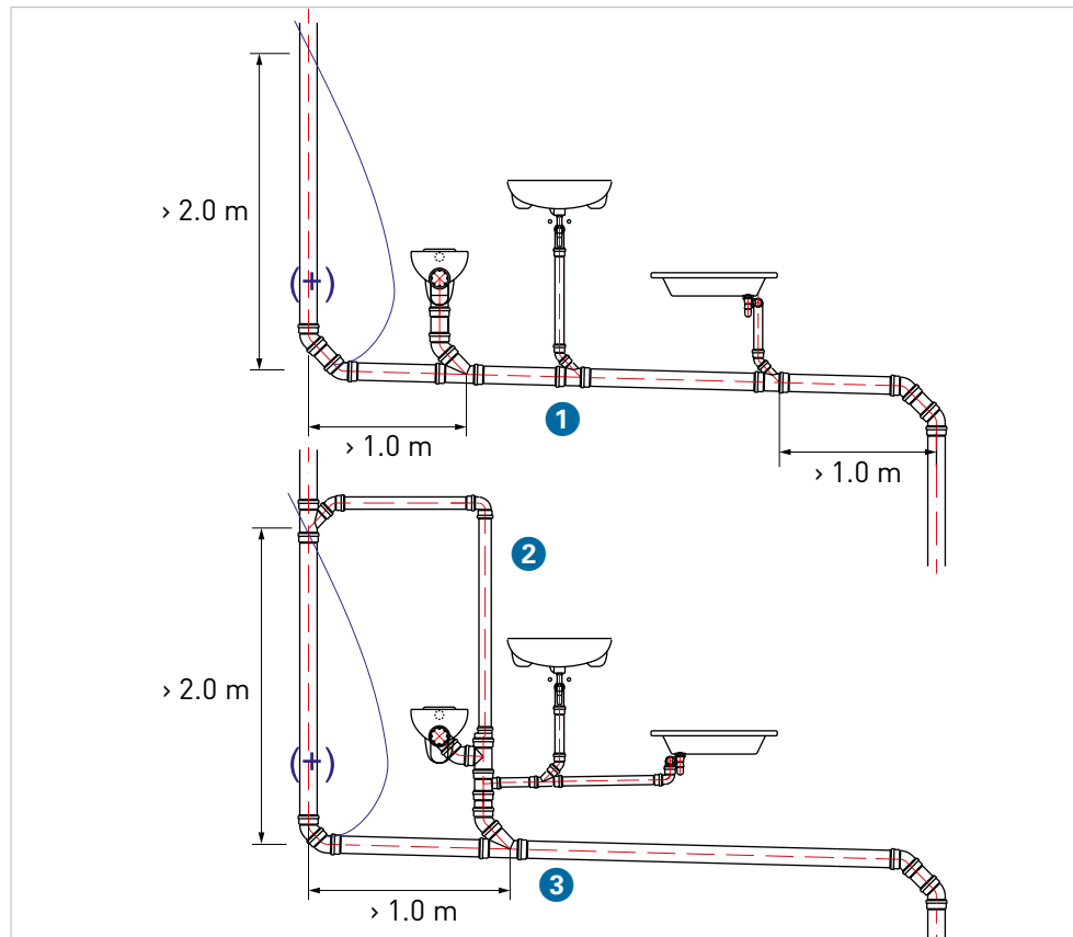
GIV.21 Connections in an area subject to critical excessive pressure
