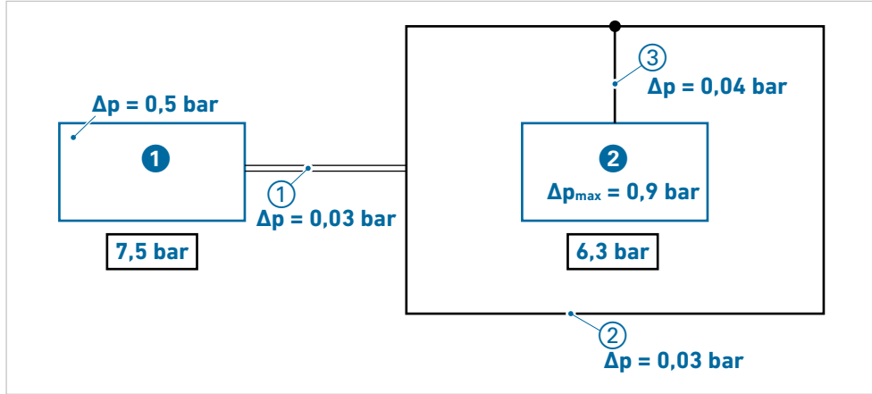
GIV.6 Total pressure loss ① Generator ② Consumer ① Main pipeline ② Distribution pipeline ③ Connecting pipeline
