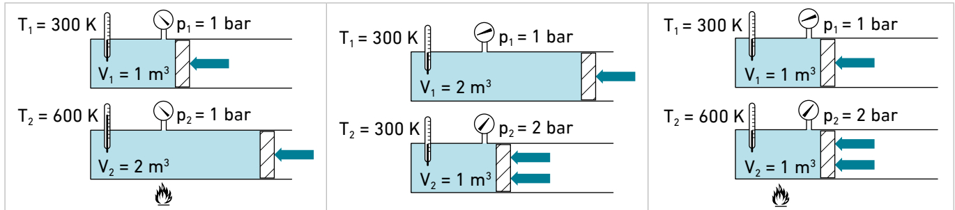
GC.12 Isobars
