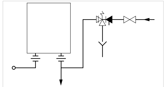
GV.21 Connection of a DHW heater – Installation diagram
