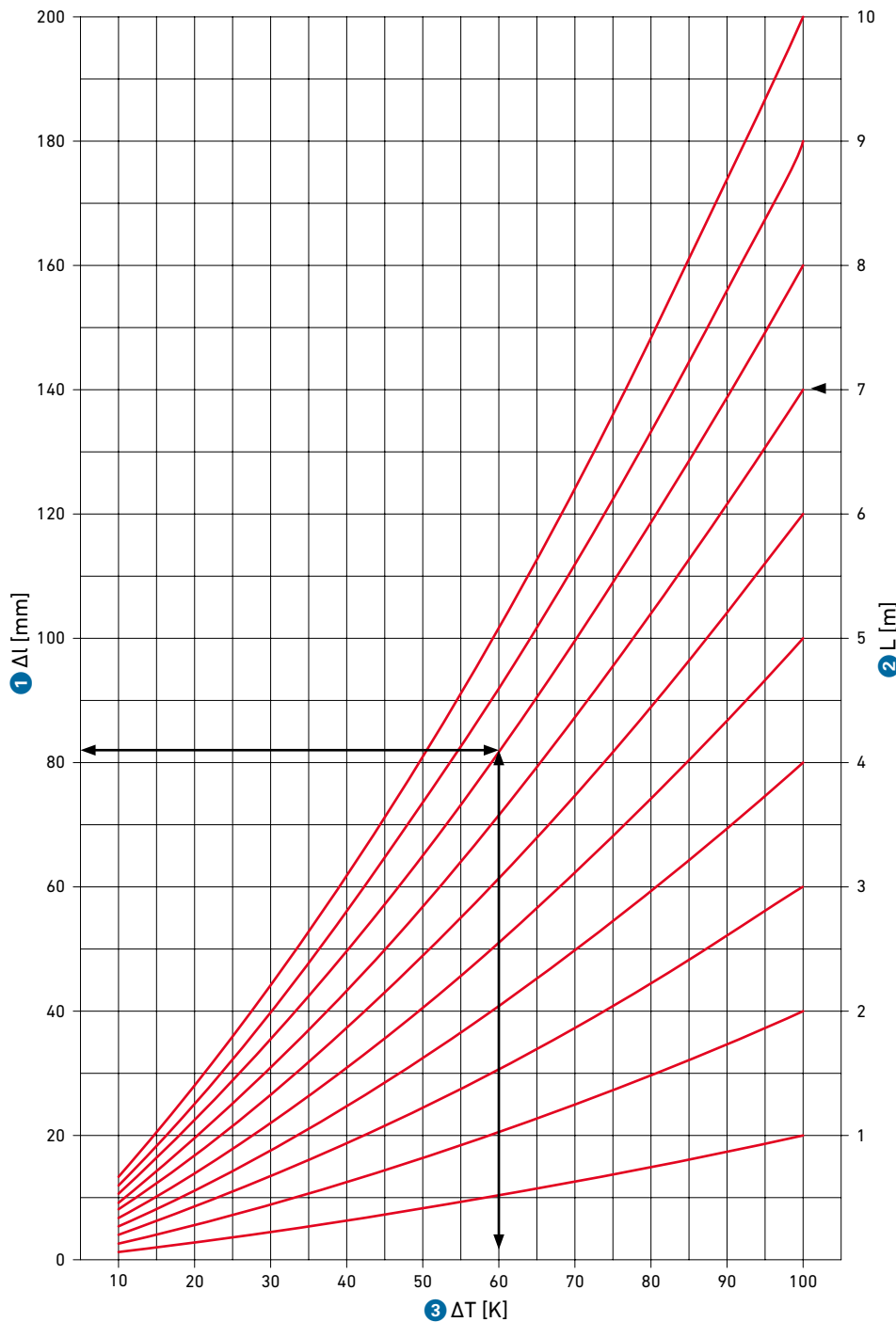
GV.10 Change in length – JRG Sanipex pipe (PE-X) with non-linear coefficient of thermal expansion Change in length Length of pipeline Temperature difference
