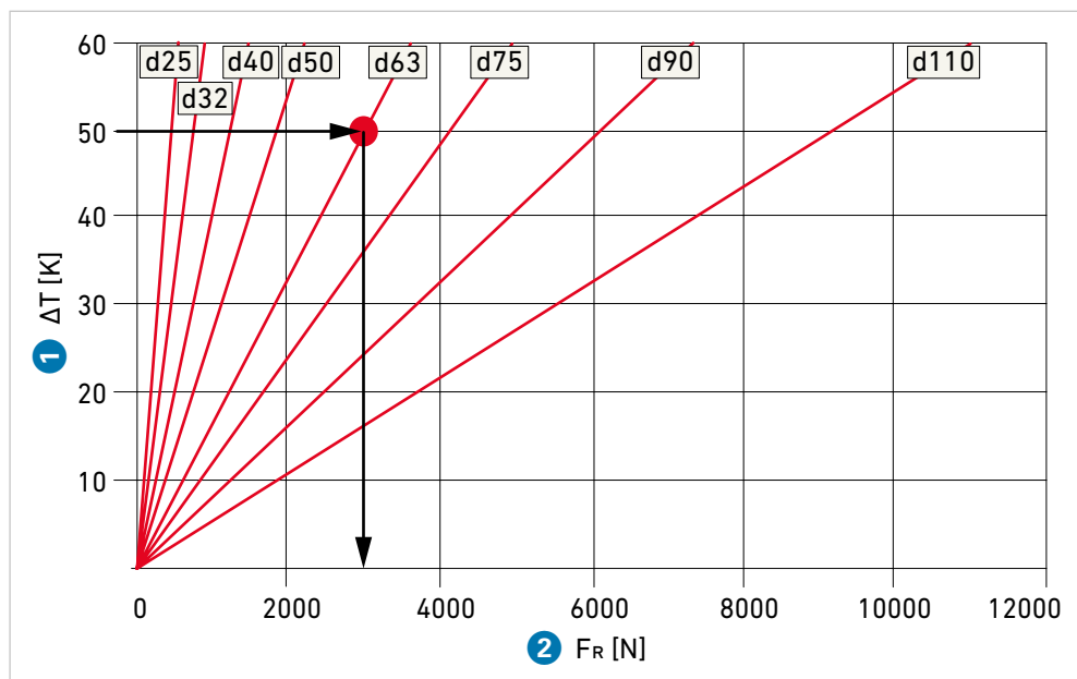
GV.34 Elongation force F_R (INSTAFLEX, PB pipe) 1 Temperature difference 2 Elongation force
