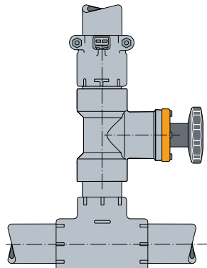
Balancing valve with HWS transition (e.g. when using riser pipes)
