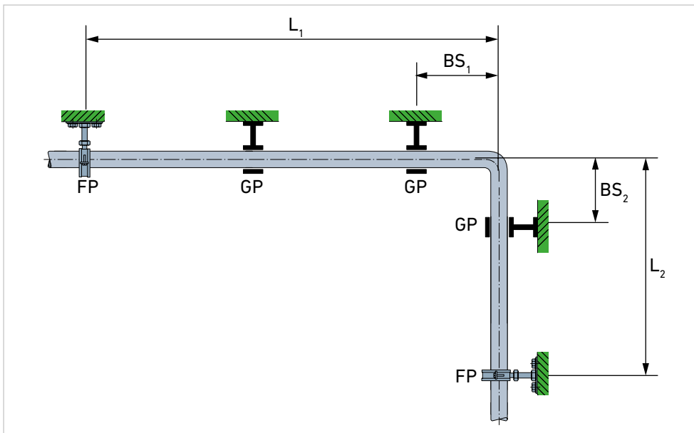
GIV.51 Flexible pipe leg FP Fixed point GP Floating point (with sliding pipe clip) BS Flexible pipe leg l Pipe length between fixed point and deflection
