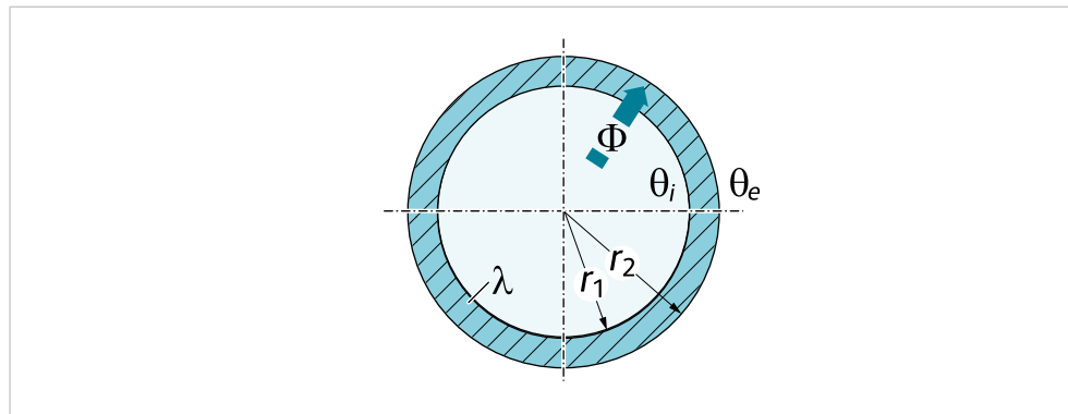
GC.17 Heat conduction through a single-layer pipe
