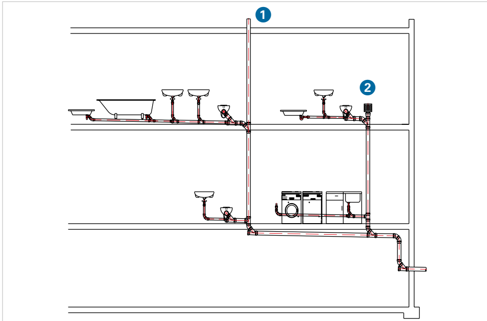
GIV.29 Use of ventilation valves in semi-detached dwelling and duplexes
