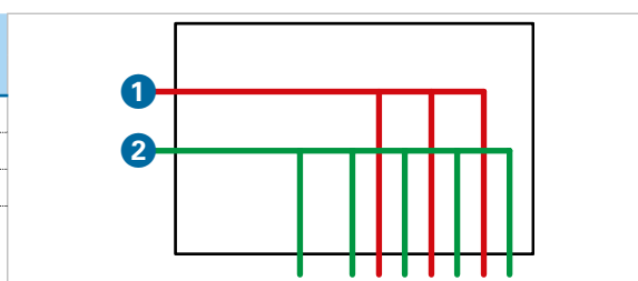
TV.2 Distributor 1 Hot water 2 Cold water
