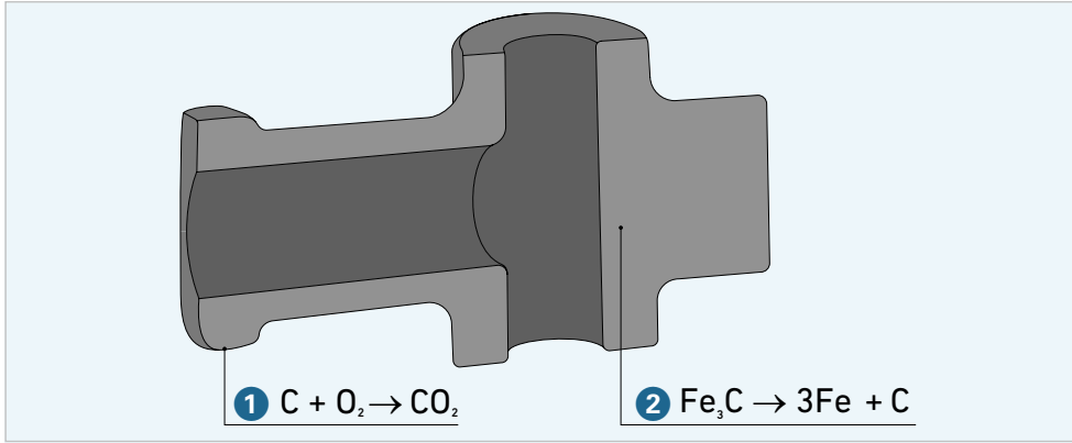
GIII.17 Processes in the casting during tempering; micrograph
