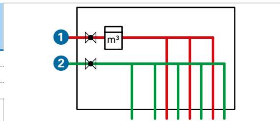
TV.9 Distributor with DHW heater water meter and shut-off valves for hot and cold water 1 Hot water 2 Cold water
