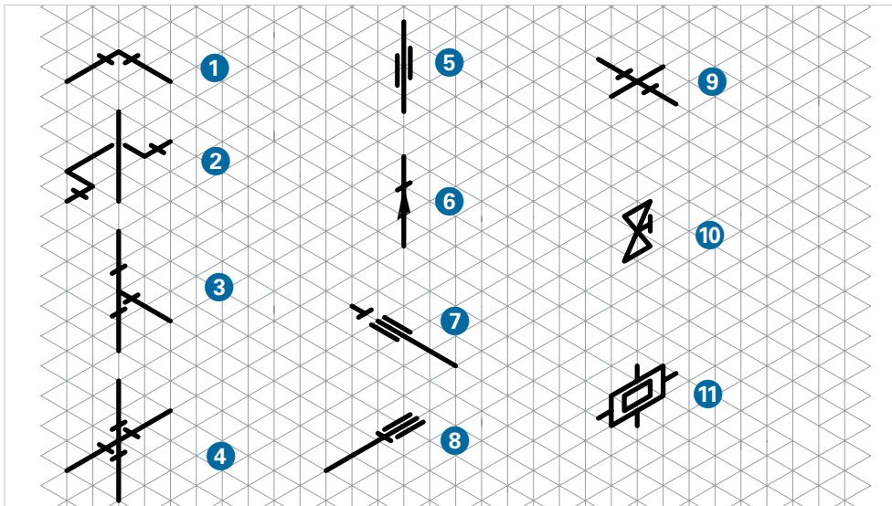
GIV.88 Symbols used to represent the routing of pipelines
