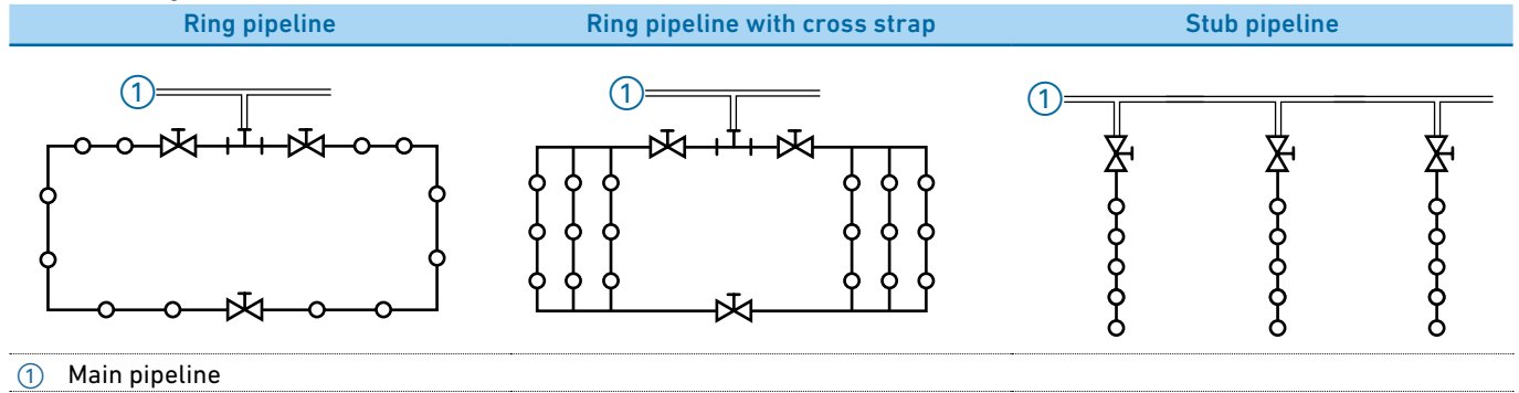
TIV.17 Planning and distribution
