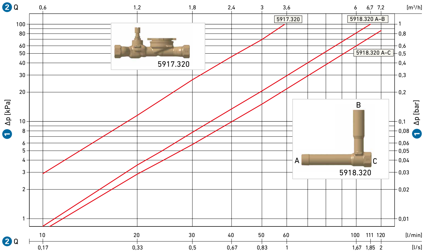
Pressure loss of individual components
