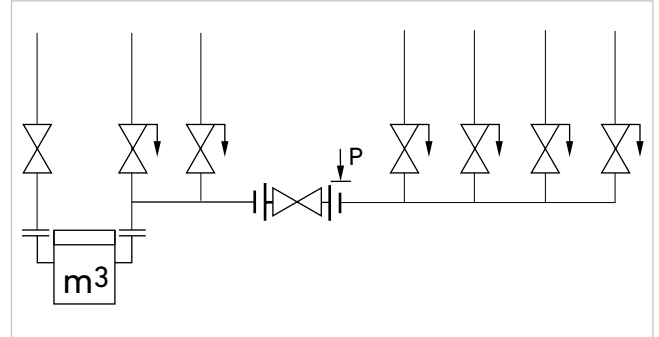
GV.33 Installation diagram
