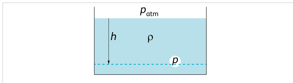
GC.26 Gravitational pressure in depth h
