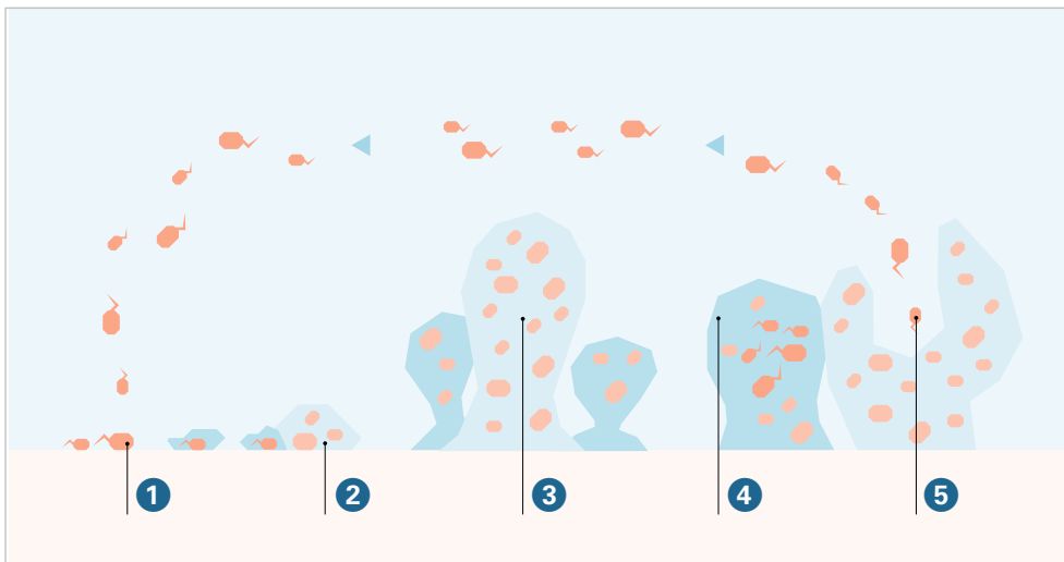
GIII.3 Formation of a biofilm
