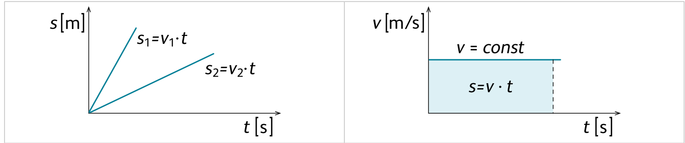
GC.4 Distance-time diagram
