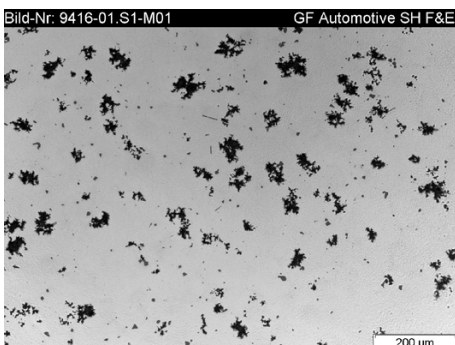
GIII.19 Black malleable iron, micrograph (unetched)
