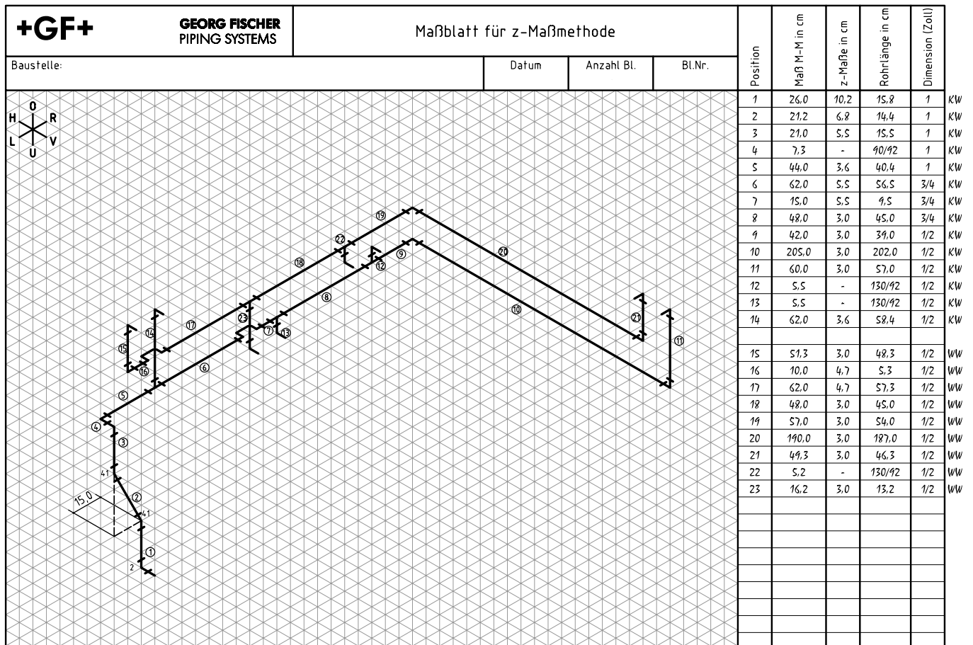
GIV.90 Examples of the filled in GF isometric graph paper
