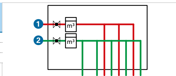
TV.10 Distributor with hot and cold water meter and shut-off valves 1 Hot water 2 Cold water
