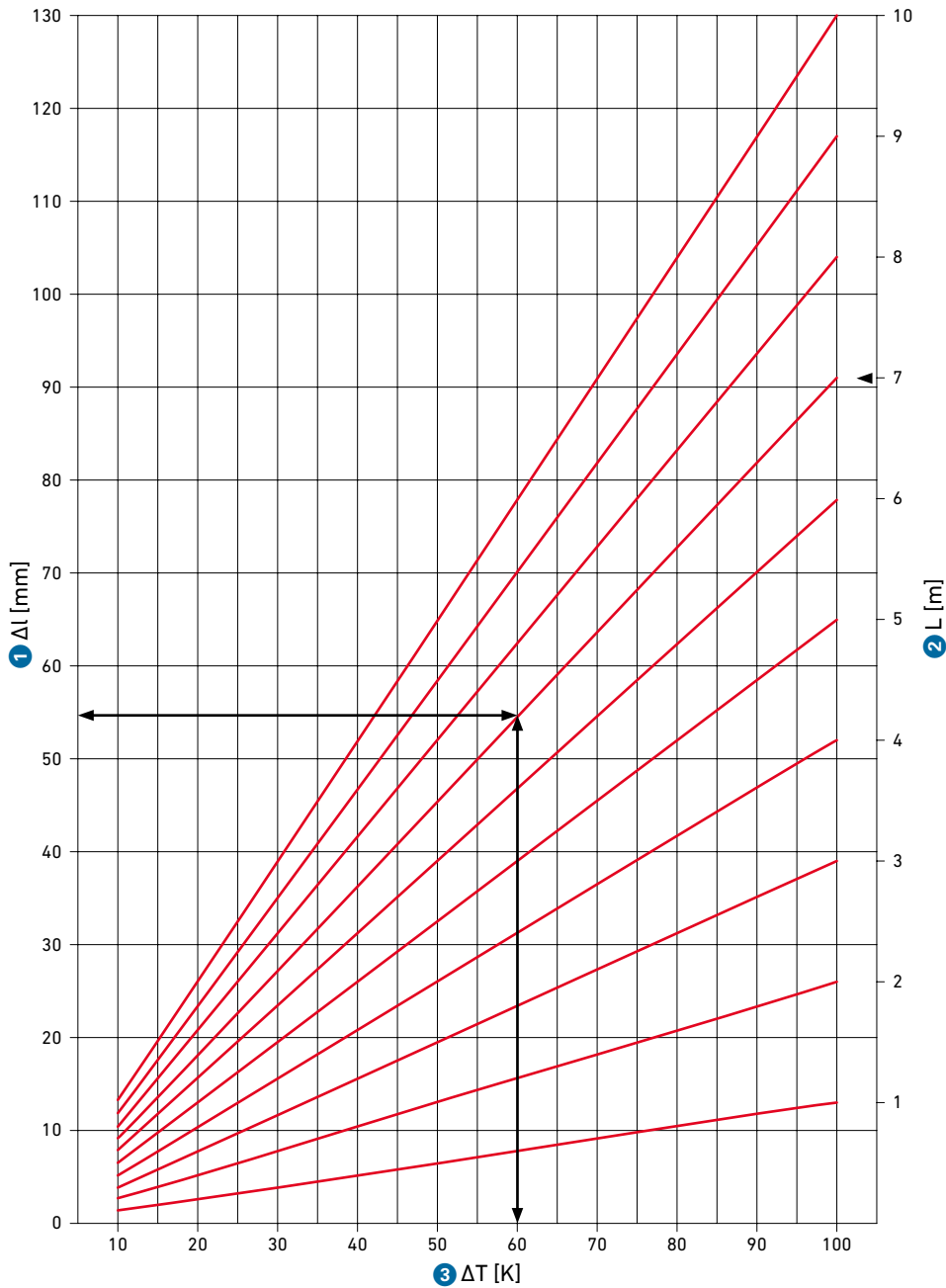
GV.10 Change in length – iFIT pipes (PB) 1 Change in length 2 Length of pipeline 3 Temperature difference
