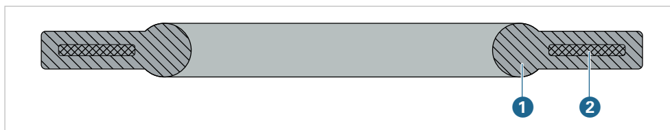
GIII.43 Gasket with steel insert
