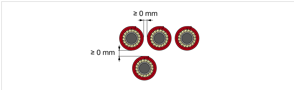
GV.22 Zero distance
