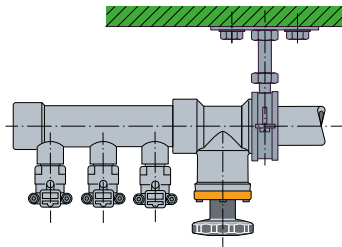
PB valve with distributor in the duct pipe shaft
