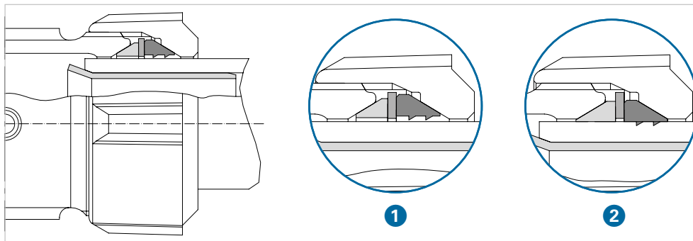
GV.5 Connection for PE- und PE-Xa-pipe ① Loose Connection ② Tightened connection
