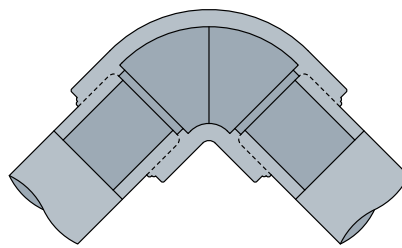
Socket fusion welding (HMS), firmly bonded, for PB and PE
