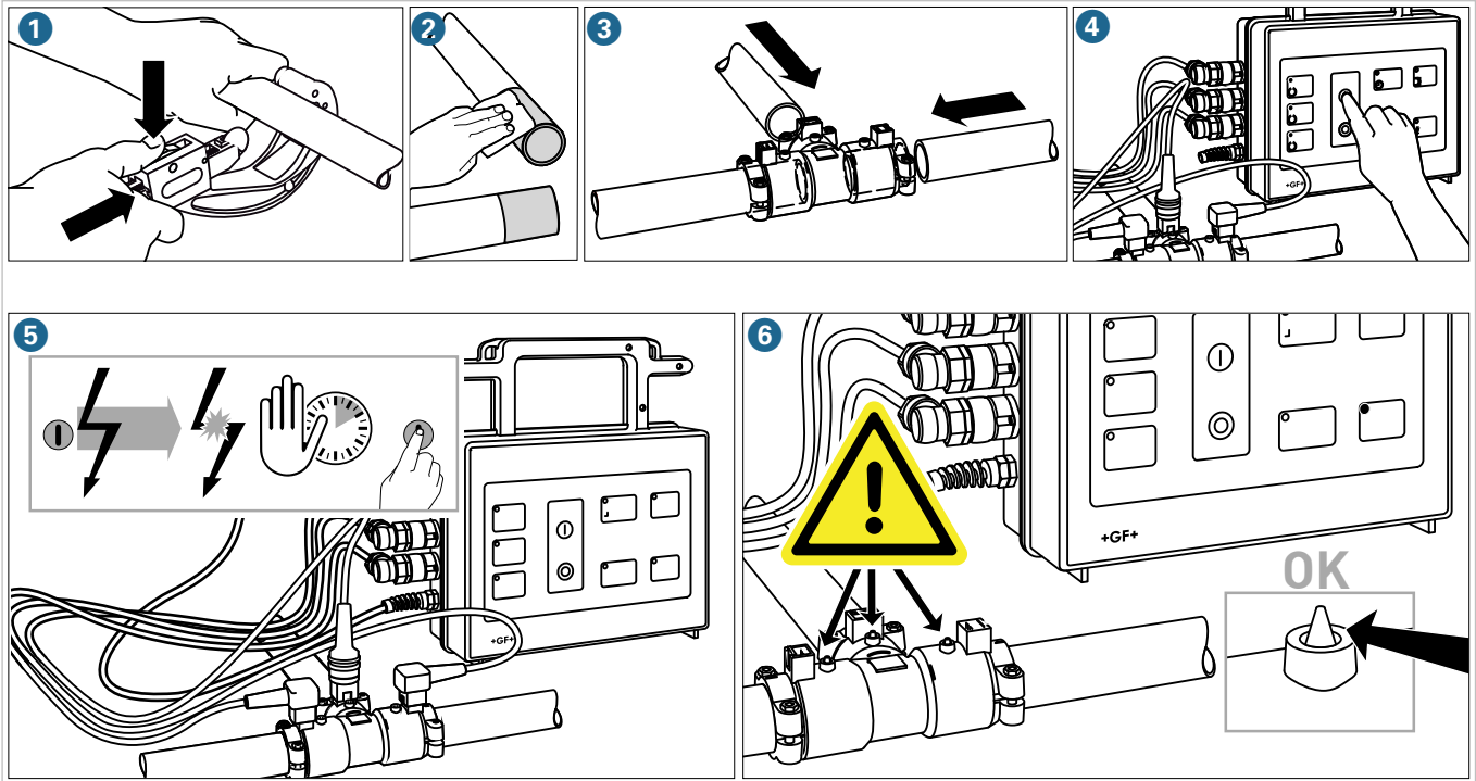
GIII.41 Fusion process
