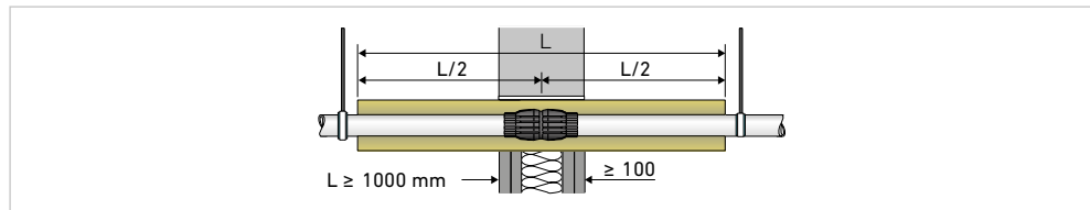
GV.21 Assembly of the JRG pipe connector
